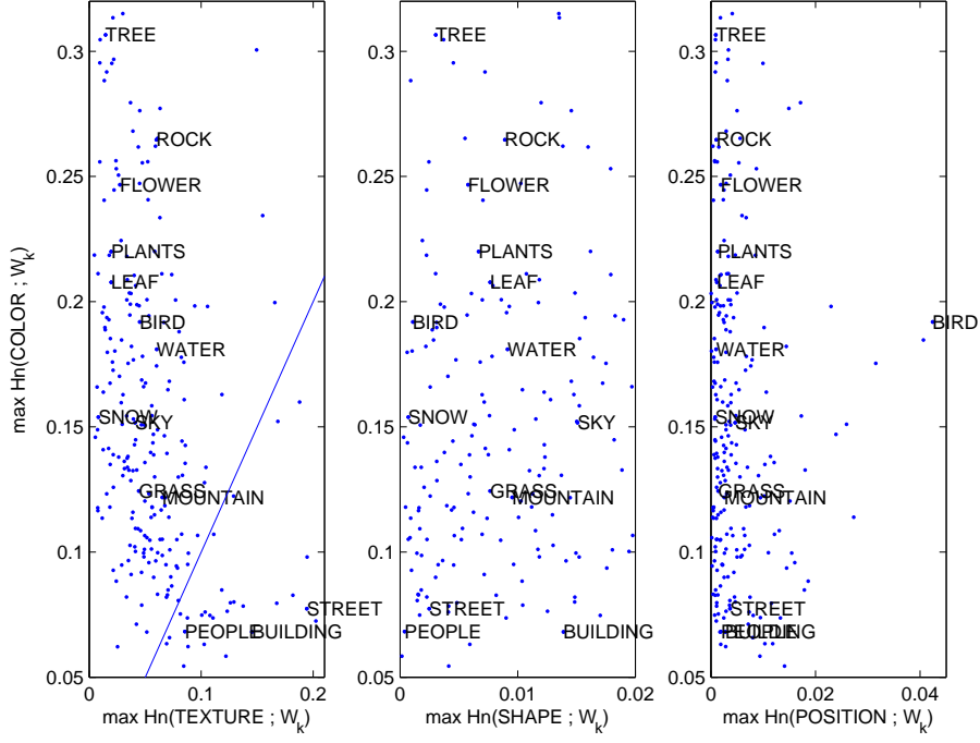
Figure 2: Maximum values of normalised estimated discrimination power Hn(x; w_k) = \hat{F}(x; w_k) / \sum_x \hat{F}(x, w_k) for COLOR, TEXTURE, SHAPE, and POSITION features sets for the 14 most frequent words of the database (other words are represented by a simple dot). Results are intuitively correct: TREE, ROCK, FLOWER, PLANTS are mostly discriminated by color; while BUILDING and STREET are more discriminated by texture. SHAPE is in average not very competitive in comparison to COLOR, neither POSITION. BIRD is the word the most discriminated by POSITION, indeed most of COREL images with a bird represent a bird in the image center.
